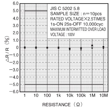
Fig. 10 Intermittent overload
