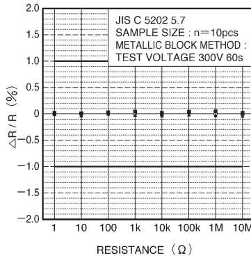
Fig. 9 Withstand voltage
